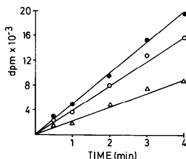
Fig.3. The effect of osmotic shock treatment of the incorporation of dThd from dTMP by cells of S. typhimurium LT 2 . Concentration of dTMP 10^{-5} M; radioactivity 12.5\text{ mCi/mmol} ; ●, untreated cells; △, treated cells; ○, treated cells supplemented with their own shock fluid after 15 min preincubation.
